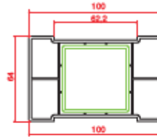
62X100 Kutu 62x100 Box
