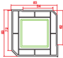
Universal Kutu Universal Box
