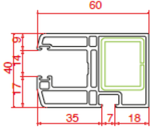
Yan Ray Profili Side Rail Guide Profile
