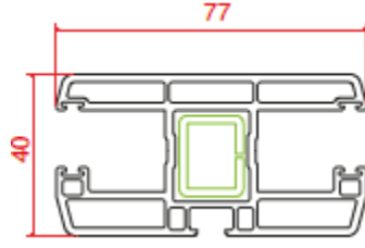
Orta Ray Profili Mullion Rail Guide Profile
