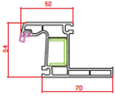
Pervazlı Kasa Architrave Frame
