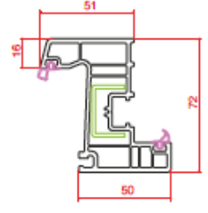
Pencere Kanat Window Sash
