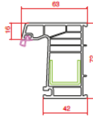
6 Odacıklı Kasa Frame 6 Chamber
