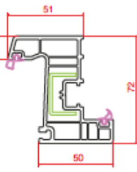
Dar Pencere Kanat Narrow Window Sash
