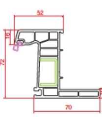
Pervazlı Kasa Architrave Frame
